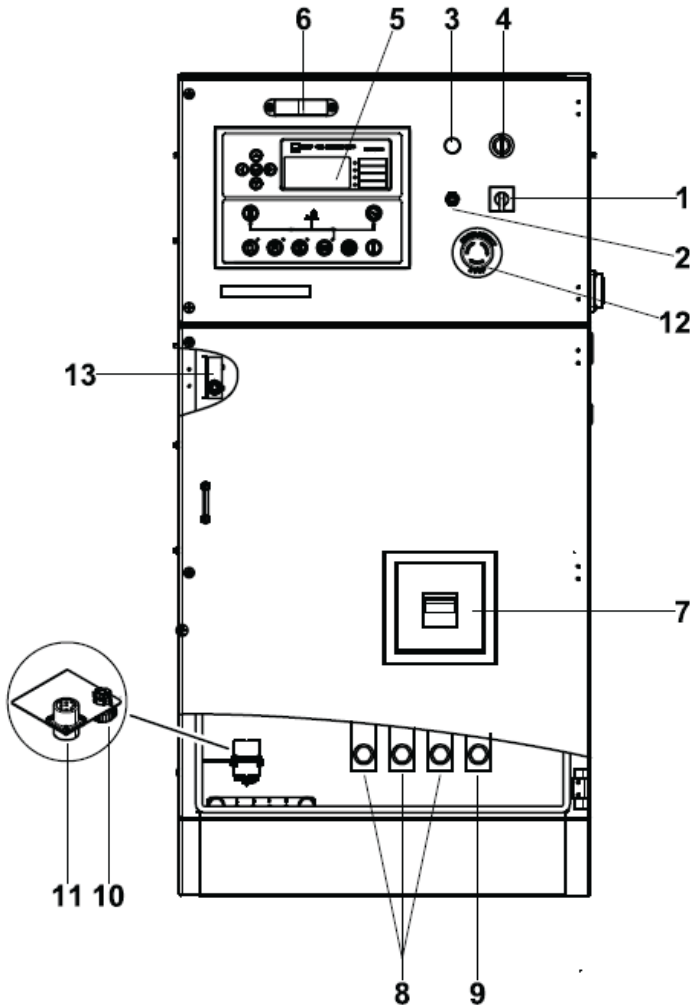
Control & Field wiring cabinet
